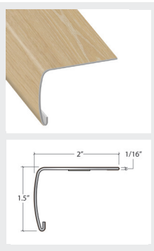
Tall Stair Nose Cap
