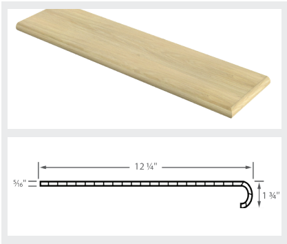
Round Stair Tread with Return
