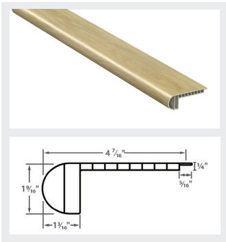
Round Flush Stair Nose
